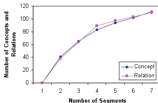
Figure 2. Graph to show that the number of concepts and relations in the corpus is becoming stationary
